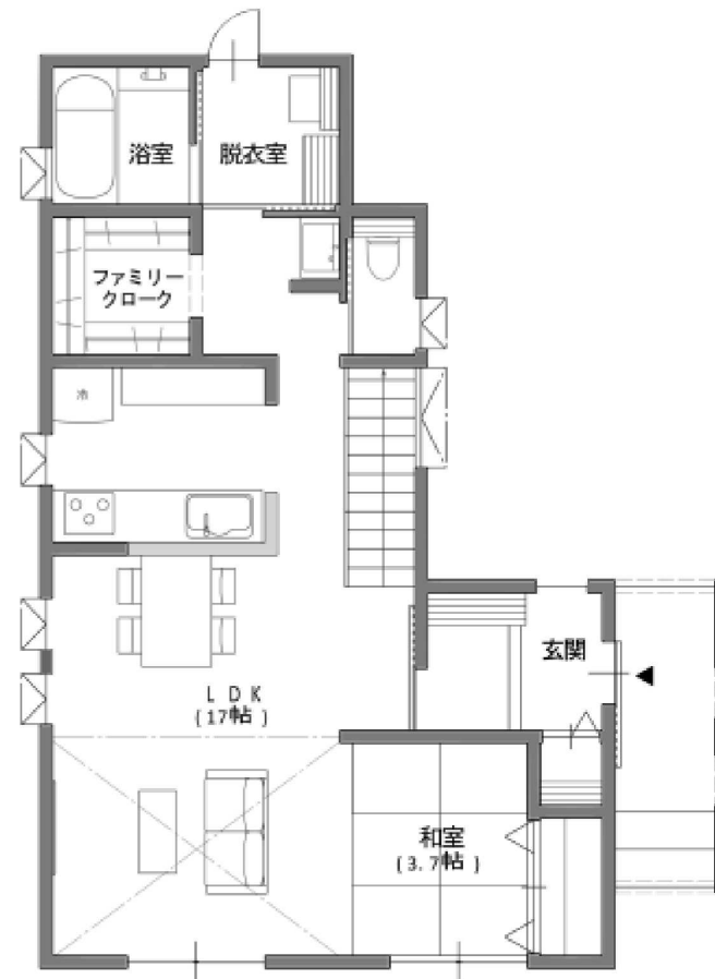
1F Plan
