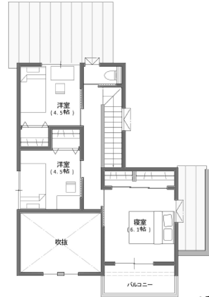
2F Plan
